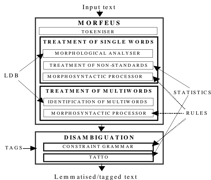
Figure 1: Architecture of EUSLEM
